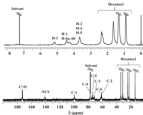
Figure 1. ^1\text{H} and ^{13}\text{C} NMR spectra of product A (compound 4a ).
